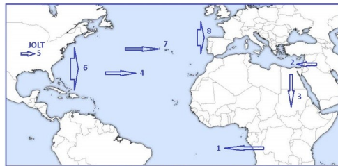
1 Africa Foot into S Atlantic 2 Rock Hook Fracture 3 Africa Drops 4 SE Portion Tugged 5 Bridge Snaps JOLT 6 SE Portion Jumps East 7 Azores Ruptures 8 Tsunami Results
