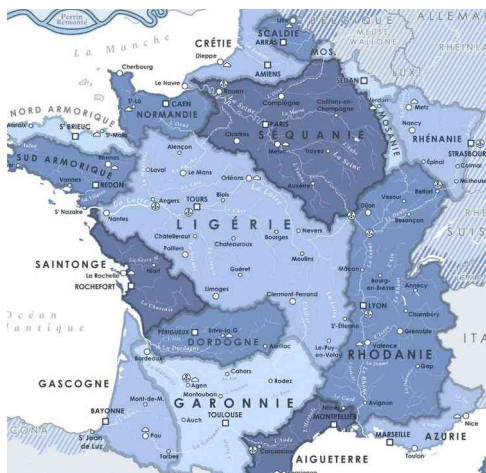
Figure 61: Bassins versants France
