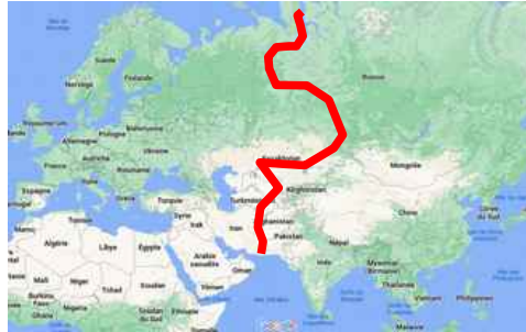
Figure 28: plaque eurasiennne coupée en 2 (Est Oural)
