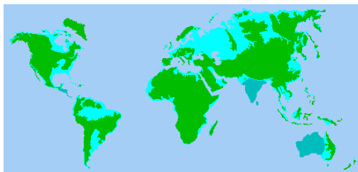
Figure 30: Montée des eaux mondiale (zetatalk)
